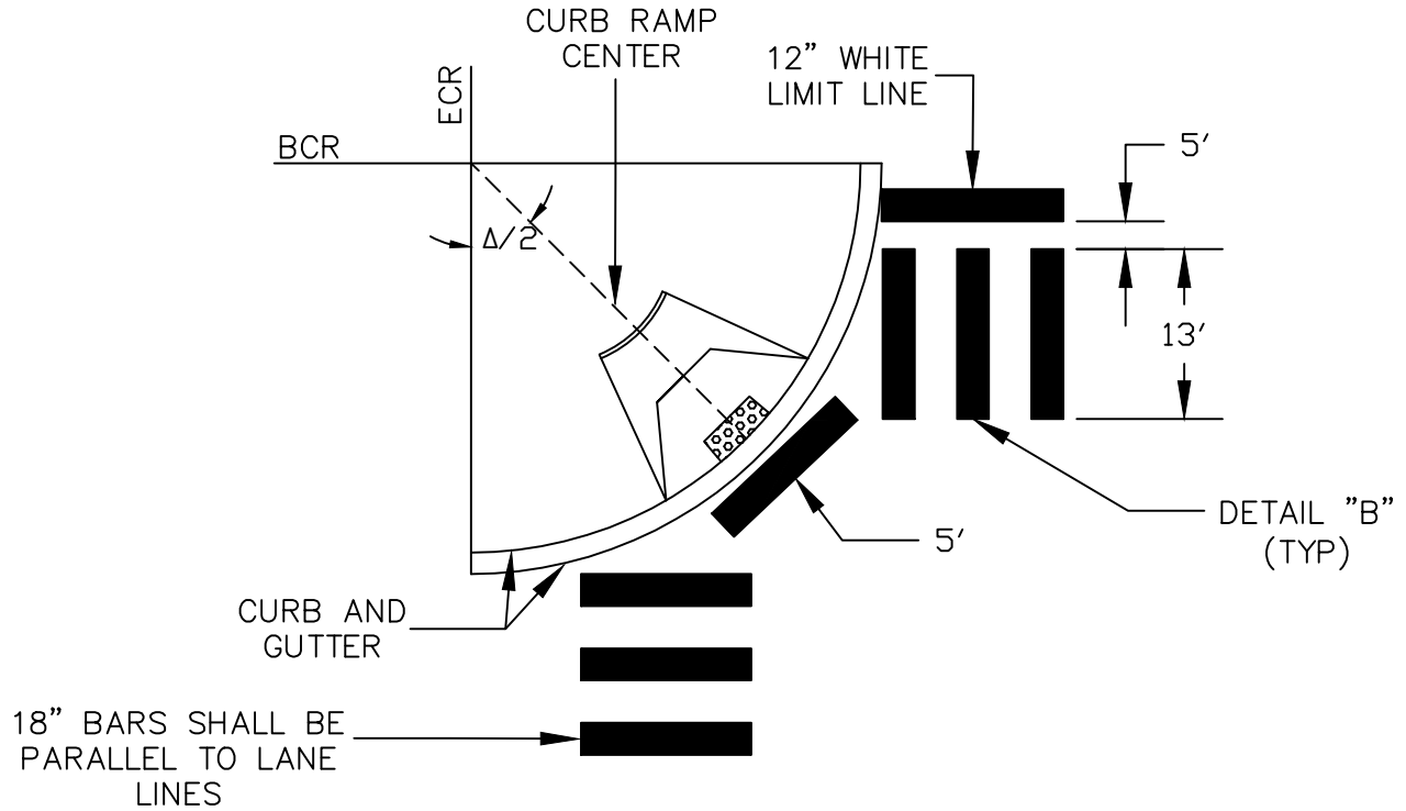
CONTINENTAL CROSSWALK (Not To Scale)
